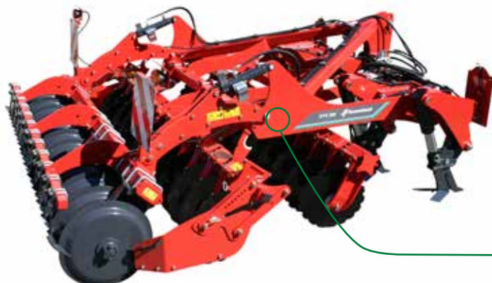
CLG-III 2.20, 2.90, 3.80, 4.70 and 5.60m; 50cm deep
